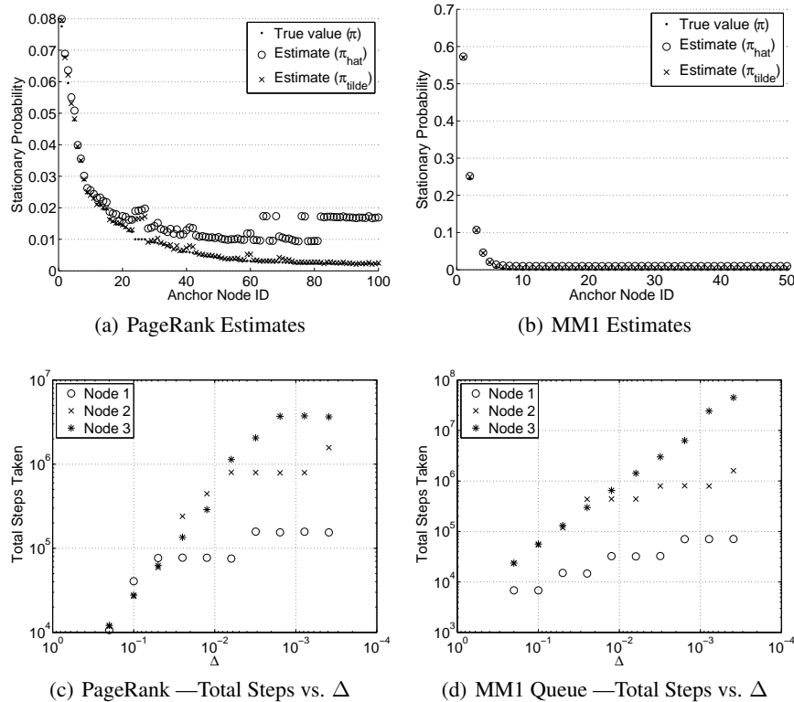
Figure 2: Simulations showing results of our algorithm applied to PageRank and MM1 Queue setting
