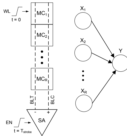
Fig. 2. A simplified critical path for small-signal sensing.
