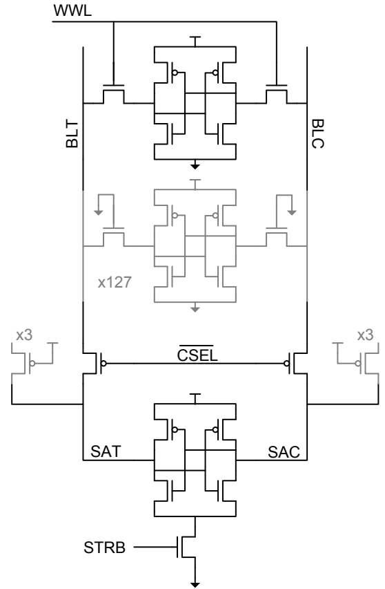
Fig. 3. Transistor level schematic of a representative memory column with 128 cells per bitline and additional multiplexing of 4 columns per sense amplifier. Precharge devices are not shown for clarity.
